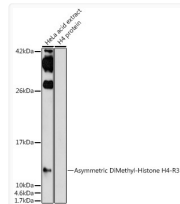
Western blot analysis of lysates from HeLa cells, using Asymmetric DiMethyl-Histone H4-R3 Rabbit polyclonal antibody (STJ29402) at 1:1000 dilution. Secondary antibody: HRP Goat Anti-Rabbit IgG (H+L) (STJS000856) at 1:10000 dilution. Lysates/proteins: 25 Mu g per lane. Blocking buffer: 3% nonfat dry milk in TBST. Detection: ECL Enhanced Kit. Exposure time: 300s.
