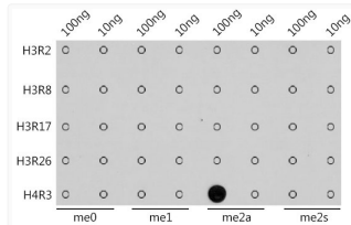
Dot-blot analysis of all sorts of methylation peptides using Asymmetric DiMethyl-Histone H4-R3 antibody (STJ29402) at 1:1000 dilution.
