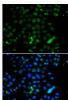
Immunofluorescence analysis of A549 cells using ELF4 antibody (STJ29260). Blue: DAPI for nuclear staining.
