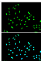
Immunofluorescence analysis of A549 cells using SMARCAD1 antibody (STJ28413). Blue: DAPI for nuclear staining.
