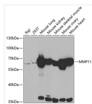
Western blot analysis of extracts of various cell lines, using MMP11 antibody (STJ24575) at 1:500 dilution. Secondary antibody: HRP Goat Anti-Rabbit IgG (H+L) (STJS000856) at 1:10000 dilution. Lysates/proteins: 25 µg per lane. Blocking buffer: 3% nonfat dry milk in TBST. Detection: ECL Basic Kit. Exposure time: 2min.
