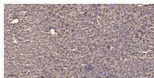
Immunohistochemical analysis of paraffin-embedded human liver cancer. 1, Antibody was diluted at 1:200 (4° overnight). STJ196059
