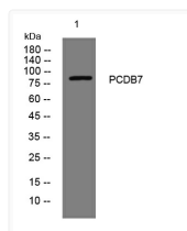
Western blot analysis of lysates from CACO2 cells, primary antibody was diluted at 1:1000, 4°C overnight STJ196059
