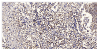
Immunohistochemical analysis of paraffin-embedded human squamous cell carcinoma of lung. 1, Antibody was diluted at STJ196031
