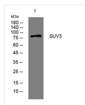
Western blot analysis of lysates from MDA-MB cells, primary antibody was diluted at 1:1000, 4° overnight STJ196031
