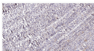
Immunohistochemical analysis of paraffin-embedded human colon cancer. 1, Antibody was diluted at 1:200 (4° overnight). STJ195151
