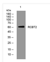
Western blot analysis of lysates from A431 cells, primary antibody was diluted at 1:1000, 4° overnight STJ195151
