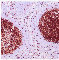
Anti-Ki-67 antibody IHC Human lymph node STJ180311
