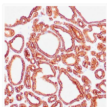
Anti-Cytokeratin 18 antibody IHC Human thyroid gland STJ180142
