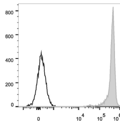
Rat thymocytes were stained with Anti-CD90.1 antibody (STJA0001083) [Used at 0.05 µg/10 6 cells dilution] (filled gray histogram). Unstained thymocytes (empty black histogram) were used as control.
