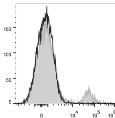
Human peripheral blood lymphocytes were stained with Anti-CD20 antibody (STJA0001053) (filled gray histogram) or Mouse IgG2b Isotype Control PE/Cy7 (empty black histogram).
