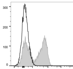
C57BL/6 murine splenocytes were stained with Anti-IgD antibody (STJA0001032) [Used at 0.02 µg/10 6 cells dilution] (filled gray histogram). Unstained splenocytes (empty black histogram) were used as control.
