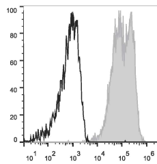
Human erythroleukemic cell line (HEL) were stained with Anti-CD90 antibody (STJA0000960) (filled gray histogram) or Mouse IgG1, κ Isotype Control (PE/Cyanine7 Conjugated) (empty black histogram).
