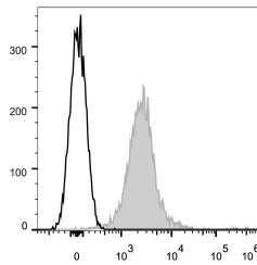
C57BL/6 murine splenocytes were stained with Anti-Mouse PD-L1 Monoclonal Antibody (APC Conjugated) [Used at 0.05 µg/10 6 cells dilution] (filled gray histogram). Unstained splenocytes (empty black histogram) were used as control.
