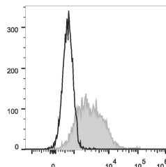
Con-A stimulated C57BL/6 splenocytes (3 days) were stained with Anti-CD279/PD-1 antibody (STJA0000821) (filled gray histogram). Unstained splenocytes (empty black histogram) were used as control.
