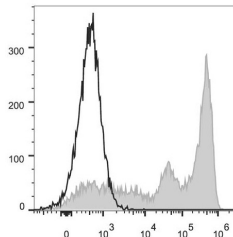
C57BL/6 murine bone marrow cells were stained with Anti-Mouse Gr-1 Monoclonal Antibody (FITC Conjugated) (Used at 0.2 µg/10 6 cells dilution) (filled gray histogram). Unstained bone marrow cells (empty black histogram) were used as control.
