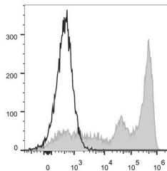
C57BL/6 murine bone marrow cells were stained with Anti-Mouse Gr-1 Monoclonal Antibody (FITC Conjugated) (filled gray histogram). Unstained bone marrow cells (empty black histogram) were used as control.
