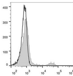
Human peripheral blood lymphocytes were stained with Anti-CD123 antibody (STJA0000708) (filled gray histogram). Unstained lymphocytes (empty black histogram) were used as control.
