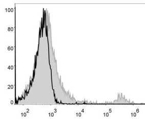
Mouse splenocytes were stained with Anti-CD8a antibody (STJA0000597) [Used at 0.2 µg/10 6 cells dilution] (filled gray histogram). Unstained splenocytes (blank black histogram) were used as control.
