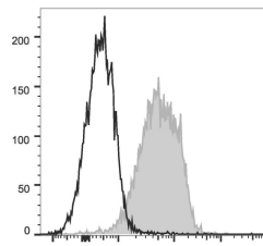
C57BL/6 murine splenocytes were stained with Anti-CD1d1 antibody (STJA0000296) (filled gray histogram). Unstained splenocytes (empty black histogram) were used as control.
