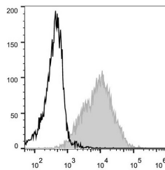
C57BL/6 murine splenocytes were stained with Anti-CD54 antibody (STJA0000230) (filled gray histogram). Unstained splenocytes (empty black histogram) were used as control.
