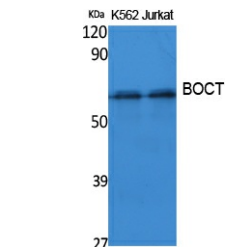
Western blot analysis of extracts from K562, Jurkat cells, using BOCT Polyclonal Antibody. Secondary antibody was diluted at 1:20000
