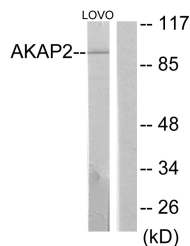
Western blot analysis of lysates from LOVO cells, using AKAP2 Antibody. The lane on the right is blocked with the synthesized peptide.
