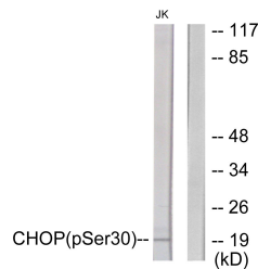
Western blot analysis of lysates from Jurkat cells treated with PMA 125ng/ml 30', using CHOP (Phospho-Ser30) antibody. The lane on the right is blocked with the phospho peptide.
