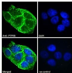
STJ72286 Immunofluorescence analysis of paraformaldehyde fixed A431 cells, permeabilized with 0.15% Triton. Primary incubation 1hr (10µg/ml) followed by Alexa Fluor 488 secondary antibody (2µg/ml), showing membrane and vesicle staining. The nuclear stain is DAPI (blue). Negative control: Unimmunized goat IgG (10µg/ml) followed by Alexa Fluor 488 secondary antibody (2µg/ml).
