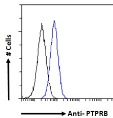
STJ72286 Flow cytometric analysis of paraformaldehyde fixed A431 cells (blue line), permeabilized with 0.5% Triton. Primary incubation 1hr (10µg/ml) followed by Alexa Fluor 488 secondary antibody (1µg/ml). IgG control: Unimmunized goat IgG (black line) followed by Alexa Fluor 488 secondary antibody.
