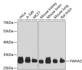
Western blot analysis of extracts of various cell lines, using YWHAZ Antibody (STJ29954) at 1:1000 dilution. Secondary antibody: HRP Goat Anti-rabbit IgG (H+L) at 1:10000 dilution. Lysates/proteins: 25µg per lane. Blocking buffer: 3% nonfat dry milk in TBST. Detection: ECL Basic Kit. Exposure time: 30s.
