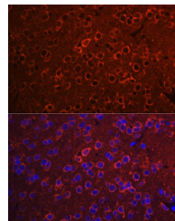
Immunofluorescence analysis of Rat brain using YWHAZ rabbit polyclonal antibody (STJ29954) at dilution of 1:100. Blue: DAPI for nuclear staining.
