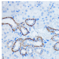
Immunohistochemistry of paraffin-embedded Rat kidney using YWHAZ rabbit polyclonal antibody (STJ29954) at dilution of 1:100 (40x lens).
