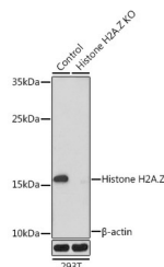
Western blot analysis of extracts from normal (control) and Histone H2A.Z rabbit polyclonal antibody knockout (KO) 293T cells, using Histone H2A.Z rabbit polyclonal antibody (STJ28697) at 1:1000 dilution. Secondary antibody: HRP Goat Anti-rabbit IgG (H+L) at 1:10000 dilution. Lysates/proteins: 25ug per lane. Blocking buffer: 3% nonfat dry milk in TBST. Detection: ECL Basic Kit. Exposure time: 1s.
