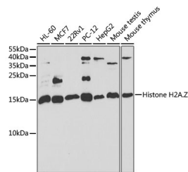
Western blot analysis of extracts of various cell lines, using H2AFZ antibody (STJ28697) at 1:1000 dilution. Secondary antibody: HRP Goat Anti-rabbit IgG (H+L) at 1:10000 dilution. Lysates/proteins: 25ug per lane. Blocking buffer: 3% nonfat dry milk in TBST. Detection: ECL Basic Kit. Exposure time: 30s.
