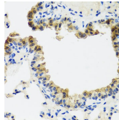
Immunohistochemistry of paraffin-embedded mouse lung using ST6GAL1 antibody (STJ28321) at dilution of 1:100 (40x lens).
