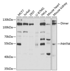
Western blot analysis of extracts of various cell lines, using P4HTM antibody (STJ27896) at 1:1000 dilution. Secondary antibody: HRP-Coat Anti-rabbit IgG (H+L) at 1:10000 dilution. Lysates/proteins: 25ug per lane. Blocking buffer: 3% nonfat dry milk in TBST. Detection: ECL Basic Kit. Exposure time: 120s.
