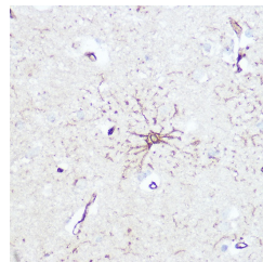
Immunohistochemistry of paraffin-embedded human brain using GFAP rabbit polyclonal antibody (STJ23770) at dilution of 1:100 (40x lens). Perform microwave antigen retrieval with 10 mM Tris/EDTA buffer pH 9.0 before commencing with immunohistochemistry staining protocol.
