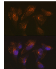
Immunofluorescence analysis of U-251 MG cells using GFAP rabbit polyclonal antibody (STJ23770) at dilution of 1:100 (40x lens). Blue: DAPI for nuclear staining.
