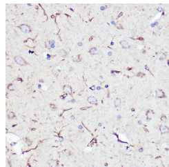
Immunohistochemistry of paraffin-embedded rat brain using GFAP rabbit polyclonal antibody (STJ23770) at dilution of 1:100 (40x lens). Perform microwave antigen retrieval with 10 mM Tris/EDTA buffer pH 9.0 before commencing with immunohistochemistry staining protocol.
