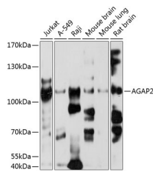
Western blot analysis of extracts of various cell lines, using AGAP2 antibody (STJ23636) at 1:1000 dilution. Secondary antibody: HRP-Goat Anti-rabbit IgG (H+L) at 1:10000 dilution. Lysates/proteins: 25µg per lane. Blocking buffer: 3% nonfat dry milk in TBST. Detection: ECL Basic Kit. Exposure time: 1s.
