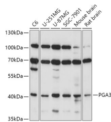
Western blot analysis of extracts of various cell lines, using PGA3 antibody (STJ119451) at 1:1000 dilution. Secondary antibody: HRP Goat Anti-rabbit IgG (H+L) at 1:10000 dilution. Lysates/proteins: 25µg per lane. Blocking buffer: 3% nonfat dry milk in TBST. Detection: ECL Basic Kit. Exposure time: 90s.
