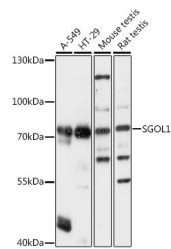
Western blot analysis of extracts of various cell lines, using SGOL1 antibody (STJ118614) at 1:1000 dilution. Secondary antibody: HRP-Coat Anti-rabbit IgG (H+L) at 1:10000 dilution. Lysates/proteins: 25µg per lane. Blocking buffer: 3% nonfat dry milk in TBST. Detection: ECL Basic Kit. Exposure time: 3s.
