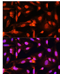
Immunofluorescence analysis of U2OS cells using SGOL1 antibody (STJ118614) at dilution of 1:100. Blue: DAPI for nuclear staining.
