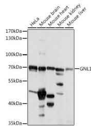
Western blot analysis of extracts of various cell lines, using GNL1 antibody (STJ118487) at 1:1000 dilution. Secondary antibody: HRP Goat Anti-rabbit IgG (H+L) at 1:10000 dilution. Lysates/proteins: 25µg per lane. Blocking buffer: 3% nonfat dry milk in TBST. Detection: ECL Basic Kit. Exposure time: 5s.
