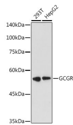
Western blot analysis of extracts of various cell lines, using GCGR antibody (STJ118008) at 1:1000 dilution. Secondary antibody: HRP Goat Anti-rabbit IgG (H+L) at 1:10000 dilution. Lysates/proteins: 25ug per lane. Blocking buffer: 3% nonfat dry milk in TBST. Detection: ECL Basic Kit. Exposure time: 180s.
