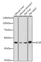
Western blot analysis of extracts of various cell lines, using GCGR antibody (STJ118008) at 1:1000 dilution. Secondary antibody: HRP Goat Anti-rabbit IgG (H+L) at 1:10000 dilution. Lysates/proteins: 25ug per lane. Blocking buffer: 3% nonfat dry milk in TBST. Detection: ECL Basic Kit. Exposure time: 10s.
