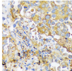
Immunohistochemistry of paraffin-embedded human lung cancer using ZDHHC18 antibody (STJ117393) at dilution of 1:100 (40x lens).
