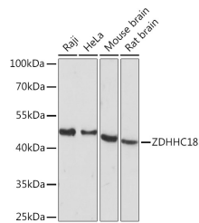
Western blot analysis of extracts of various cell lines, using ZDHHC18 rabbit polyclonal antibody (STJ117393) at 1:1000 dilution. Secondary antibody: HRP Goat Anti-rabbit IgG (H+L) at 1:10000 dilution. Lysates/proteins: 25µg per lane. Blocking buffer: 3% nonfat dry milk in TBST. Detection: ECL Basic Kit. Exposure time: 50s.
