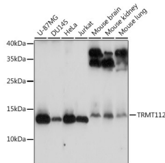
Western blot analysis of extracts of various cell lines, using TRMT112 antibody (STJ116522) at 1:3000 dilution. Secondary antibody: HRP Goat Anti-rabbit IgG (H+L) at 1:10000 dilution. Lysates/proteins: 25ug per lane. Blocking buffer: 3% nonfat dry milk in TBST. Detection: ECL Basic Kit. Exposure time: 90s.
