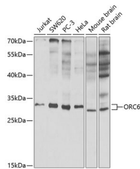
Western blot analysis of extracts of various cell lines, using ORC6 antibody (STJ116279) at 1:1000 dilution. Secondary antibody: HRP Goat Anti-rabbit IgG (H+L) at 1:10000 dilution. Lysates/proteins: 25µg per lane. Blocking buffer: 3% nonfat dry milk in TBST. Detection: ECL Basic Kit. Exposure time: 30s.
