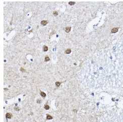
Immunohistochemistry of paraffin-embedded human brain using ORC6 rabbit polyclonal antibody (STJ116279) at dilution of 1:200 (40x lens). Perform high pressure antigen retrieval with 10 mM citrate buffer pH 6.0 before commencing with immunohistochemistry staining protocol.
