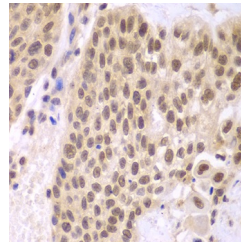
Immunohistochemistry of paraffin-embedded human lung cancer using CSNK2A2 antibody (STJ115442) at dilution of 1:100 (40x lens).
