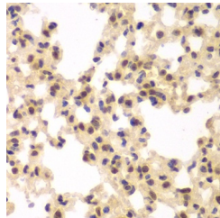
Immunohistochemistry of paraffin-embedded rat lung using CSNK2A2 antibody (STJ115442) at dilution of 1:100 (40x lens).
