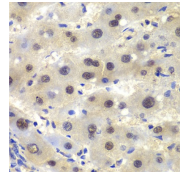
Immunohistochemistry of paraffin-embedded human liver cancer using CSNK2A2 antibody (STJ115442) at dilution of 1:100 (40x lens).
