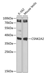
Western blot analysis of extracts of various cell lines, using CSNK2A2 antibody (STJ115442) at 1:1000 dilution. Secondary antibody: HRP Goat Anti-rabbit IgG (H+L) at 1:10000 dilution. Lysates/proteins: 25ug per lane. Blocking buffer: 3% nonfat dry milk in TBST.
