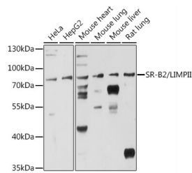
Western blot analysis of extracts of various cell lines, using SR-B2/LIMP2 antibody (STJ114596) at 1:3000 dilution. Secondary antibody: HRP Goat Anti-rabbit IgG (H+L) at 1:10000 dilution. Lysates/proteins: 25ug per lane. Blocking buffer: 3% nonfat dry milk in TBST. Detection: ECL Basic Kit. Exposure time: 30s.
