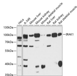
Western blot analysis of extracts of various cell lines, using IRAK1 antibody (STJ114498) at 1:3000 dilution. Secondary antibody: HRP Goat Anti-rabbit IgG (H+L) at 1:10000 dilution. Lysates/proteins: 25ug per lane. Blocking buffer: 3% nonfat dry milk in TBST. Detection: ECL Basic Kit. Exposure time: 5s.
