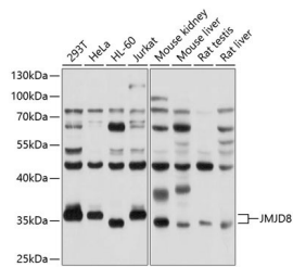
Western blot analysis of extracts of various cell lines, using JMJD8 antibody (STJ112502) at 1:1000 dilution. Secondary antibody: HRP Goat Anti-rabbit IgG (H+L) at 1:10000 dilution. Lysates/proteins: 25µg per lane. Blocking buffer: 3% nonfat dry milk in TBST. Detection: ECL Basic Kit. Exposure time: 3s.
