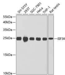
Western blot analysis of extracts of various cell lines, using EIF3K antibody (STJ112010) at 1:1000 dilution. Secondary antibody: HRP Goat Anti-rabbit IgG (H+L) at 1:10000 dilution. Lysates/proteins: 25µg per lane. Blocking buffer: 3% nonfat dry milk in TBST. Detection: ECL Basic Kit. Exposure time: 90s.
