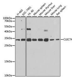
Western blot analysis of extracts of various cell lines, using CLEC7A antibody (STJ111925) at 1:1000 dilution. Secondary antibody: HRP Goat Anti-rabbit IgG (H+L) at 1:10000 dilution. Lysates/proteins: 25µg per lane. Blocking buffer: 3% nonfat dry milk in TBST. Detection: ECL Basic Kit. Exposure time: 10s.
