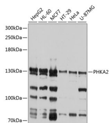
Western blot analysis of extracts of various cell lines, using PHKA2 antibody (STJ111771) at 1:1000 dilution. Secondary antibody: HRP-Goat Anti-rabbit IgG (H+L) at 1:10000 dilution. Lysates/proteins: 25µg per lane. Blocking buffer: 3% nonfat dry milk in TBST. Detection: ECL Basic Kit. Exposure time: 5s.
