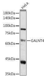
Western blot analysis of extracts of HeLa cells, using GALNT4 antibody (STJ11103560) at 1:1000 dilution. Secondary antibody: HRP Goat Anti-rabbit IgG (H+L) at 1:10000 dilution. Lysates/proteins: 25ug per lane. Blocking buffer: 3% nonfat dry milk in TBST. Detection: ECL Basic Kit. Exposure time: 180s.
