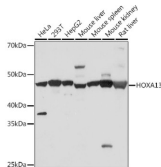
Western blot analysis of extracts of various cell lines, using HOXA13 rabbit monoclonal antibody (STJ11102493) at 1:500 dilution. Secondary antibody: HRP Goat Anti-rabbit IgG (H+L) at 1:10000 dilution. Lysates/proteins: 25µg per lane. Blocking buffer: 3% nonfat dry milk in TBST. Detection: ECL Basic Kit. Exposure time: 5s.
