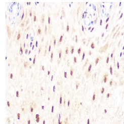
Immunohistochemistry of paraffin-embedded human esophageal using DP1/TFDP1 rabbit monoclonal antibody (STJ11102295) at dilution of 1:100 (40x lens).
