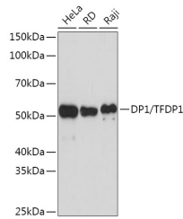
Western blot analysis of extracts of various cell lines, using DP1/TFDP1 rabbit monoclonal antibody (STJ11102295) at 1:1000 dilution. Secondary antibody: HRP Goat Anti-rabbit IgG (H+L) at 1:10000 dilution. Lysates/proteins: 25µg per lane. Blocking buffer: 3% nonfat dry milk in TBST. Detection: ECL Basic Kit. Exposure time: 60s.
