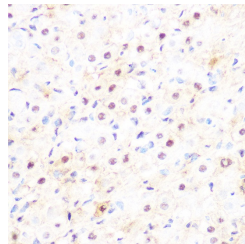
Immunohistochemistry of paraffin-embedded rat ovary using DP1/TFDP1 rabbit monoclonal antibody (STJ11102295) at dilution of 1:100 (40x lens).
