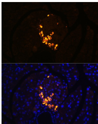
Immunofluorescence analysis of rat pancreas using GLP2 antibody (STJ11102221) at dilution of 1:100. Blue: DAPI for nuclear staining.
