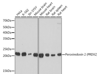
Western blot analysis of extracts of various cell lines, using Peroxiredoxin 2 (PRDX2) rabbit monoclonal antibody (STJ11102040) at 1:1000 dilution. Secondary antibody: HRP Goat Anti-rabbit IgG (H+L) at 1:10000 dilution. Lysates/proteins: 25µg per lane. Blocking buffer: 3% nonfat dry milk in TBST. Detection: ECL Basic Kit. Exposure time: 1s.
